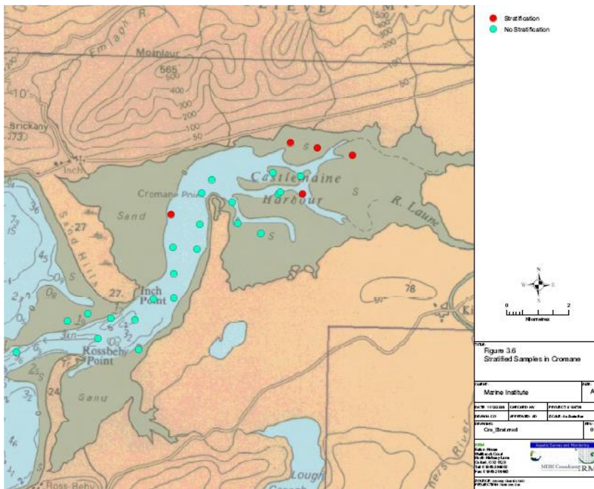
Figure 3 Distribution of stratified and non-stratified sediment conditions in grab samples in the sub-tidal channel of inner Castlemaine Harbour
